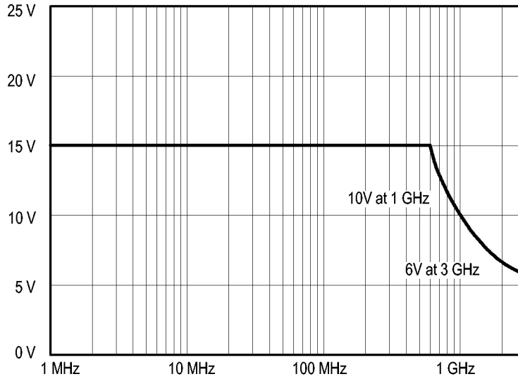
Figure 3: Typical Non-Destructive Peak Voltage Derating versus Frequency
